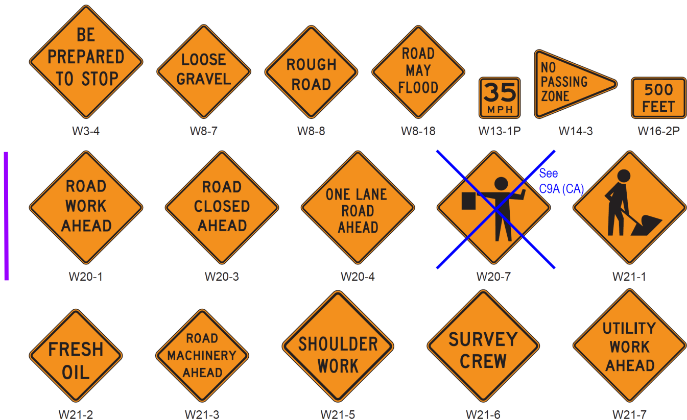
Figure 5G-1. Temporary Traffic Control Signs and Plaques on Low-Volume Roads
